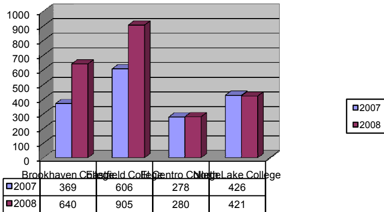
Cohort Head Count
